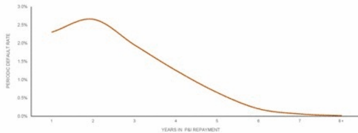
Estimated Loss Emergence Curve – Loans in P&I
